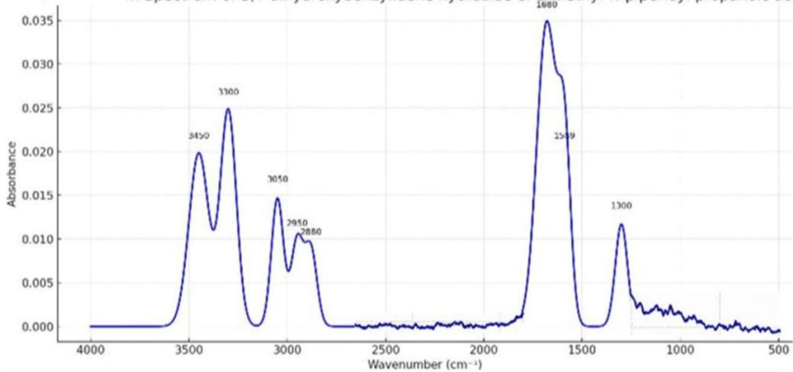
IR Spectrum of 3,4-dihydroxybenzylidene hydrazide of \alpha -methyl-N-piperidyl propanoic acid
